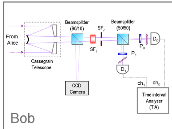
Figure 3. Bob's module. SF_1 and SF_2 are a set of spectral filters and a spatial filter, respectively; P_0 and P_1 are high extinction-ratio polarisers; M_1 is a high-reflectivity mirror; and D_0 and D_1 are single-photon detectors.
