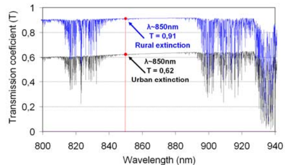
Figure 1. Comparison of the transmission coefficient T as a function of wavelength for a horizontal path of 1 km for two types of aerosol: one commonly found in urban areas and another characteristic from rural locations. Results were calculated using an atmospheric transmission simulation code (Modtran4.0)
